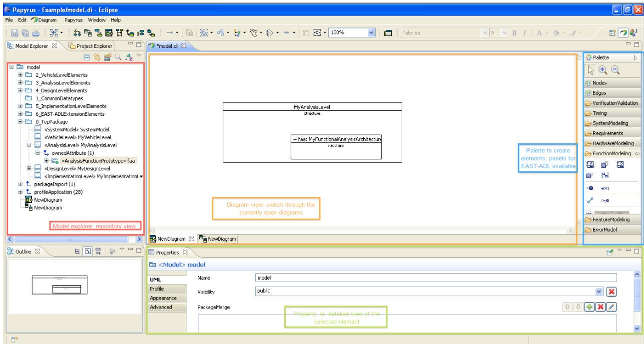
Figure 3: The most important views of a Papyrus model
