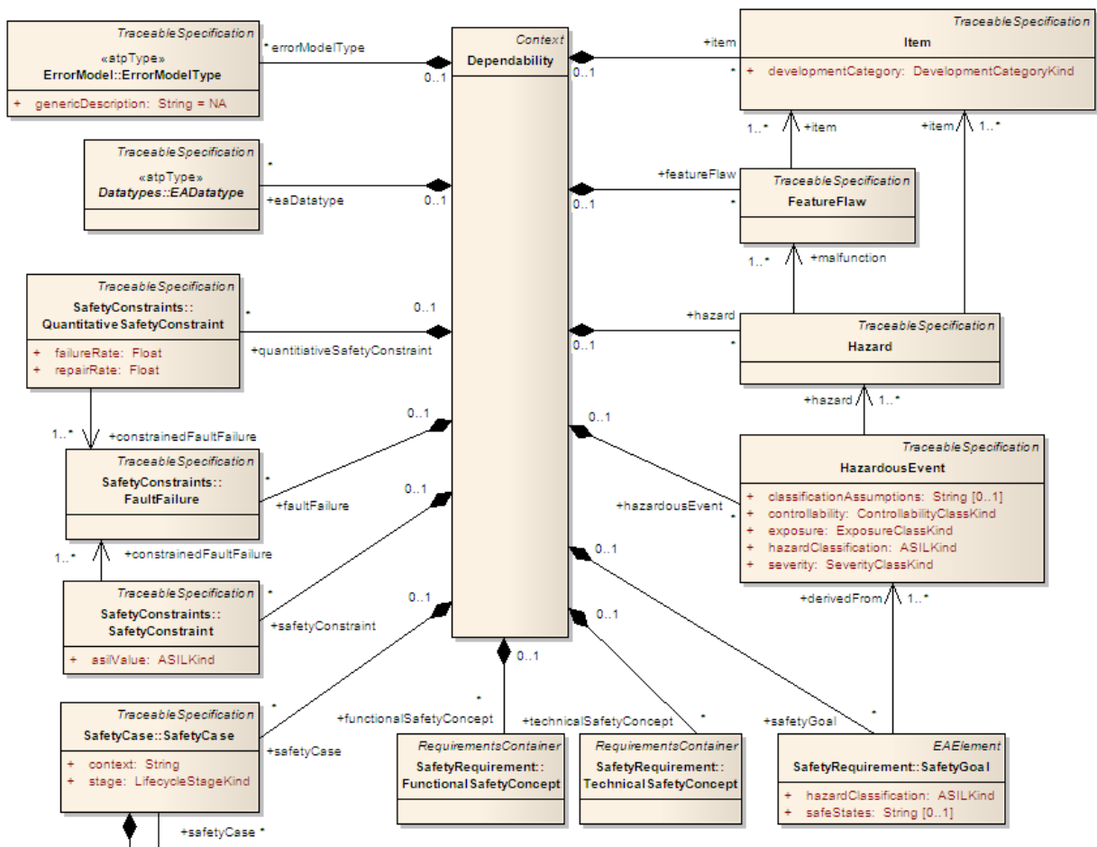
Figure 27. Diagram for organization of dependability related information.
