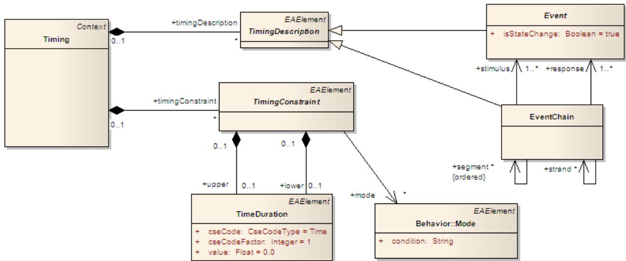
Figure 23. Diagram for the extensions of EAST-ADL abstraction layers with timing information. Timing description and timing constraints are contained in elements dedicated to the abstraction level.
