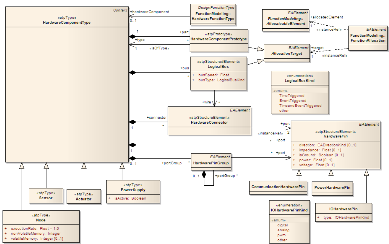
Figure 8. Diagram for HardwareModeling.
