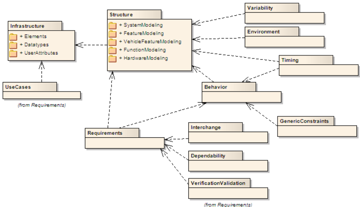
Figure 1. This diagram shows dependencies between packages in the domain model. All packages except the AUTOSAR package depend on the EAST-ADL Infrastructure package.
