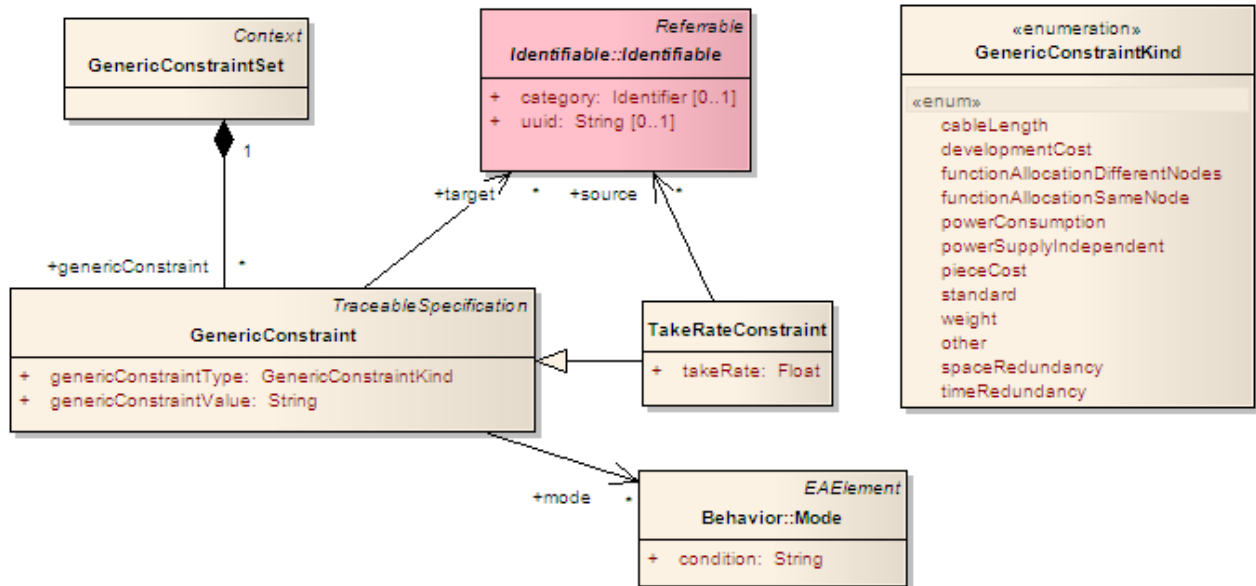
Figure 34. Diagram of GenericConstraint.
