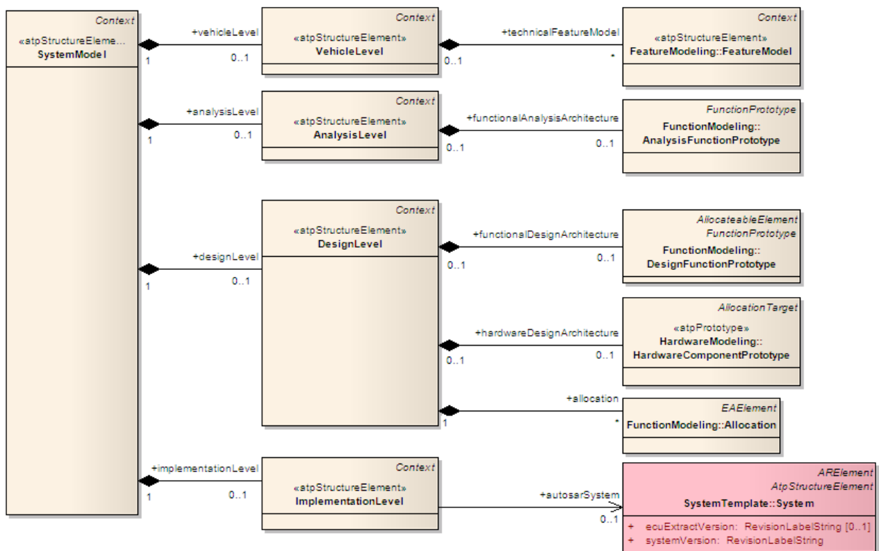
Figure 3. Diagram for SystemModel. Note how the ImplementationLevel refers to the System from the AUTOSAR SystemTemplate.
