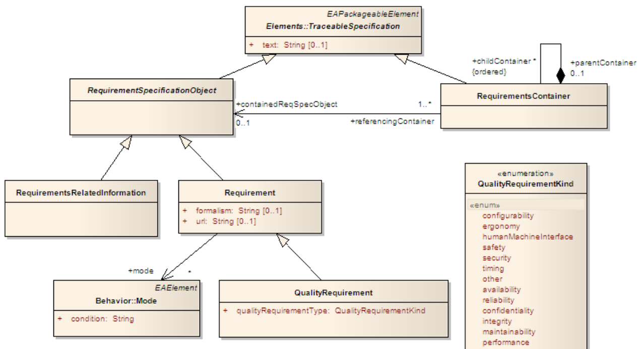
Figure 15. Diagram for Requirements overview.
