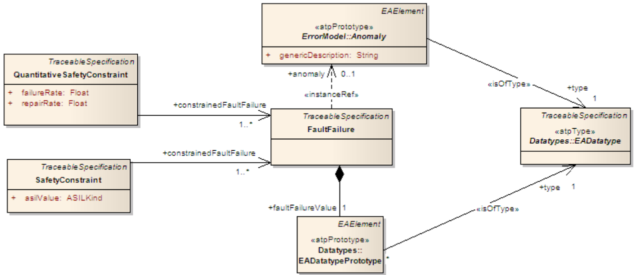
Figure 31. Diagram for SafetyConstraints.
