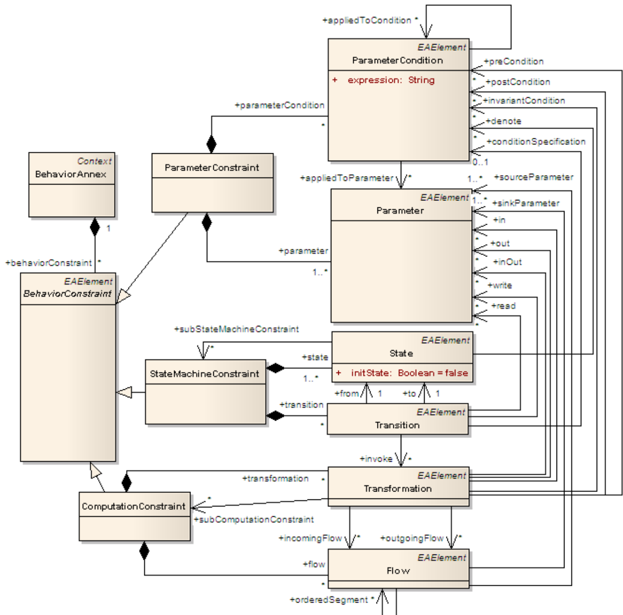
Figure 41. Diagram for organization in BehaviorConstraints.
