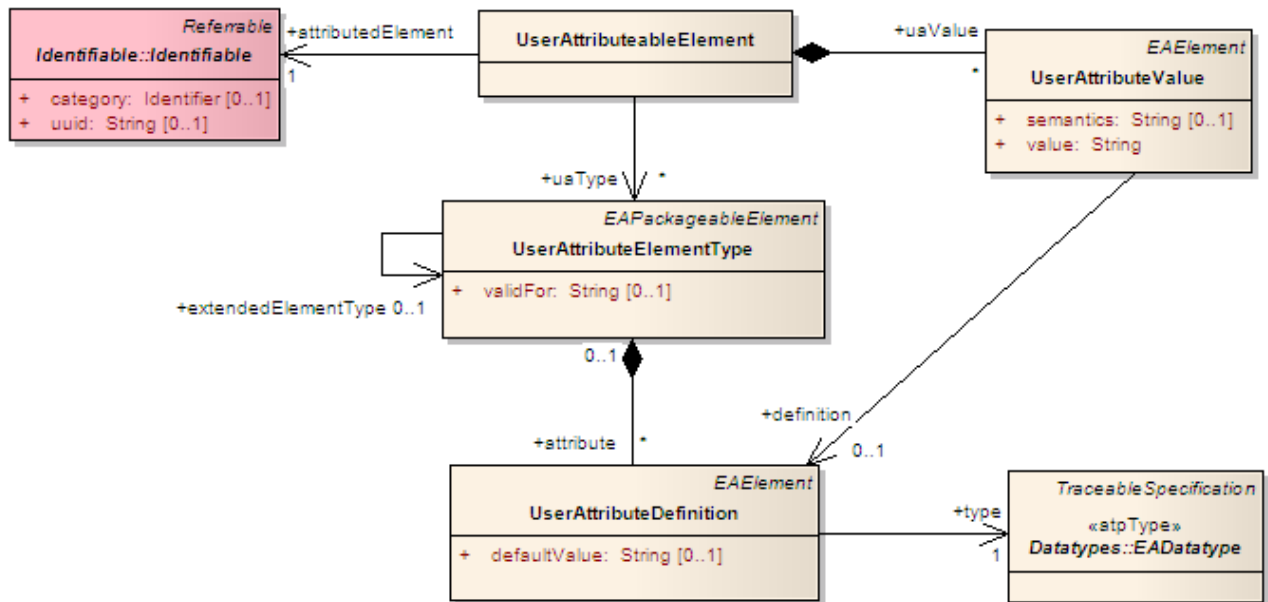
Figure 38. Diagram for User Attributes.
