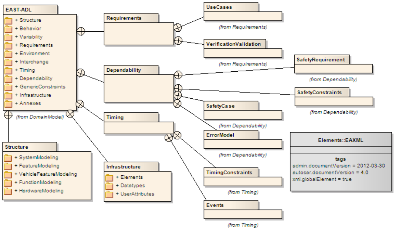
Figure 2. Packages in the EAST-ADL domain model.
