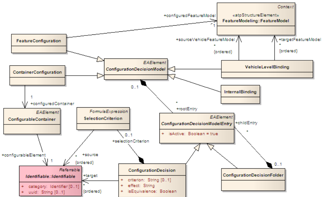
Figure 14. Diagram depicting the elements for configuration modeling.
