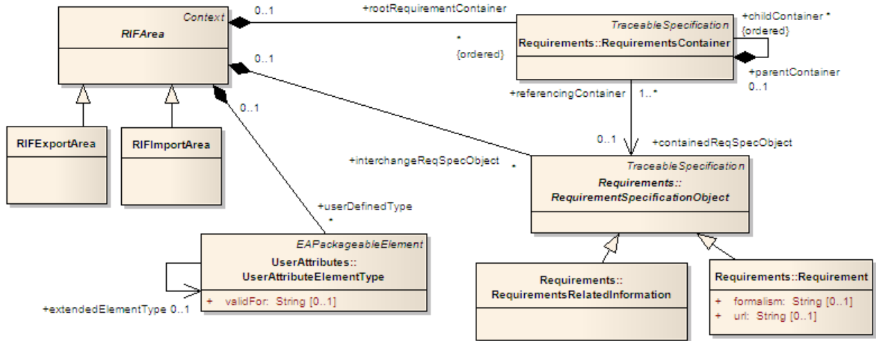
Figure 21. Diagram for RIF Area.
