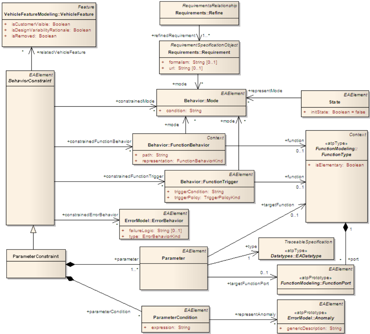
Figure 40. Diagram for dependencies of BehaviorConstraints.
